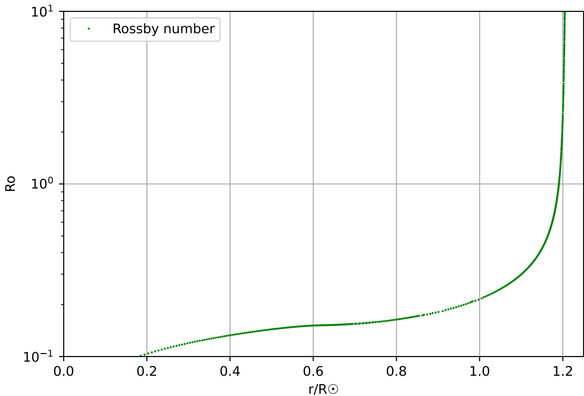
Rossby number, profile 103, age 1.1 \times 10^7
